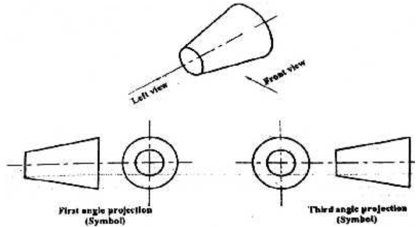
Symbol of 1 st Angle Symbol of 3 rd Angle
